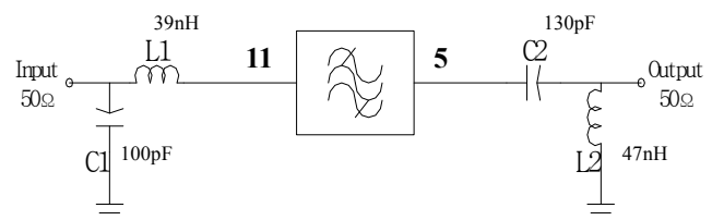
Matching Schematic
