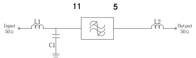
Matching Schematic
